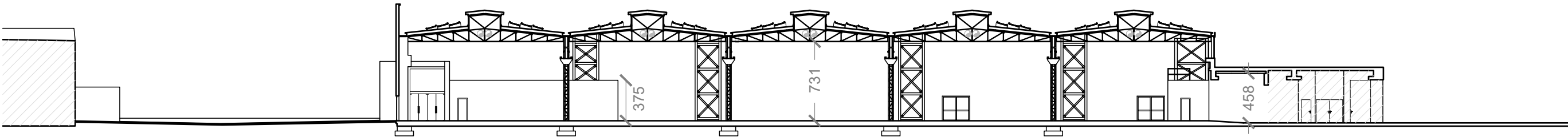
section AA'
